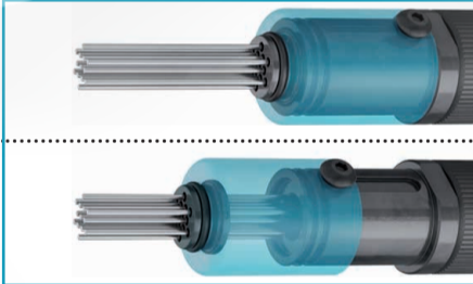
Adjustable needle carriage with integrated needle guide ensures long service life
